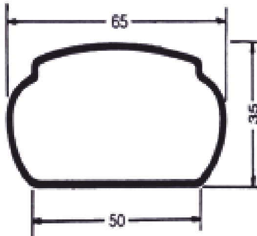
MT6 - 15/10=kg/ml 2,15
